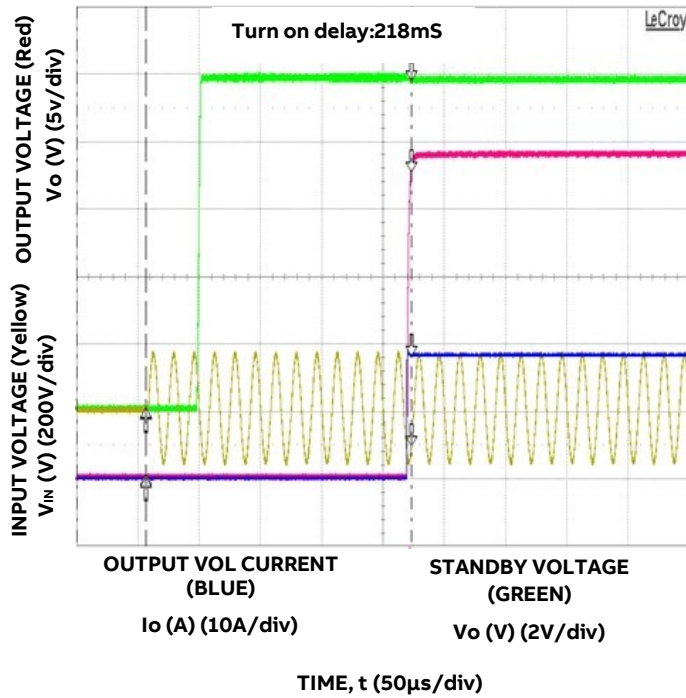
Figure 4. Typical Start-up (VIN = 115Vac, Full Load)
