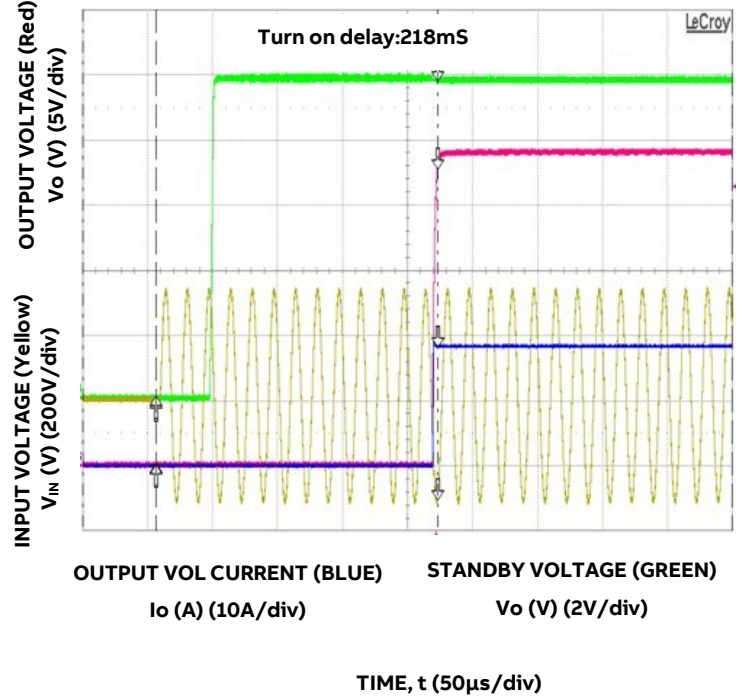
Figure 5. Typical Start-up (VIN = 230V, Full Load)
