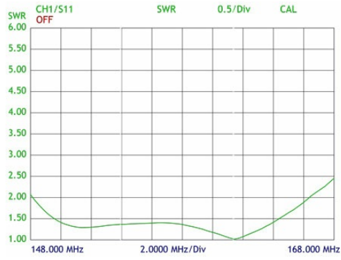
TYPICAL GAIN AND VSWR CURVE
