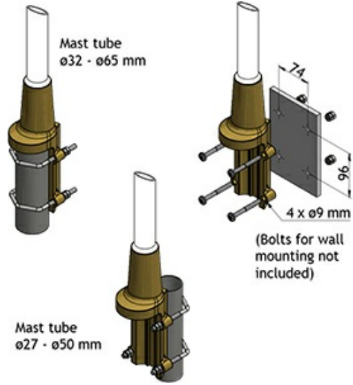
MULTI-PURPOSE MOUNTING BRACKET
