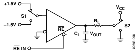
Figure 8. Receiver Enable/Disable
