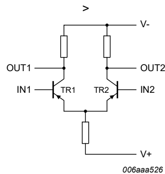
Fig. 10. Differential amplifier
