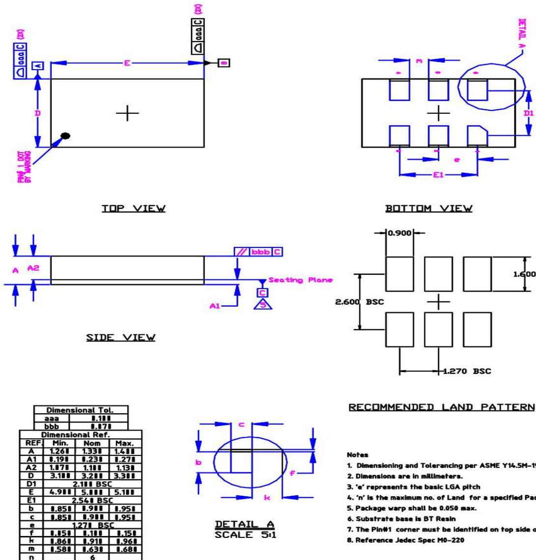
6-Pin LGA (5x3.2mm)
