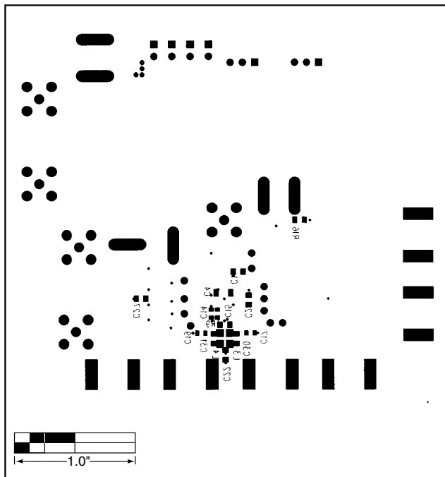
Figure 6. MAX2510 EV Kit PC Board Layout—Bottom Silkscreen and Pad Placement
