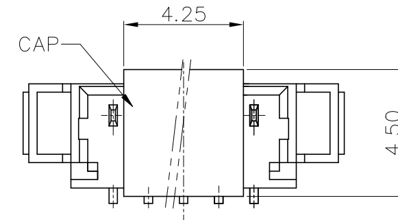
ASSEMBLY CAP
