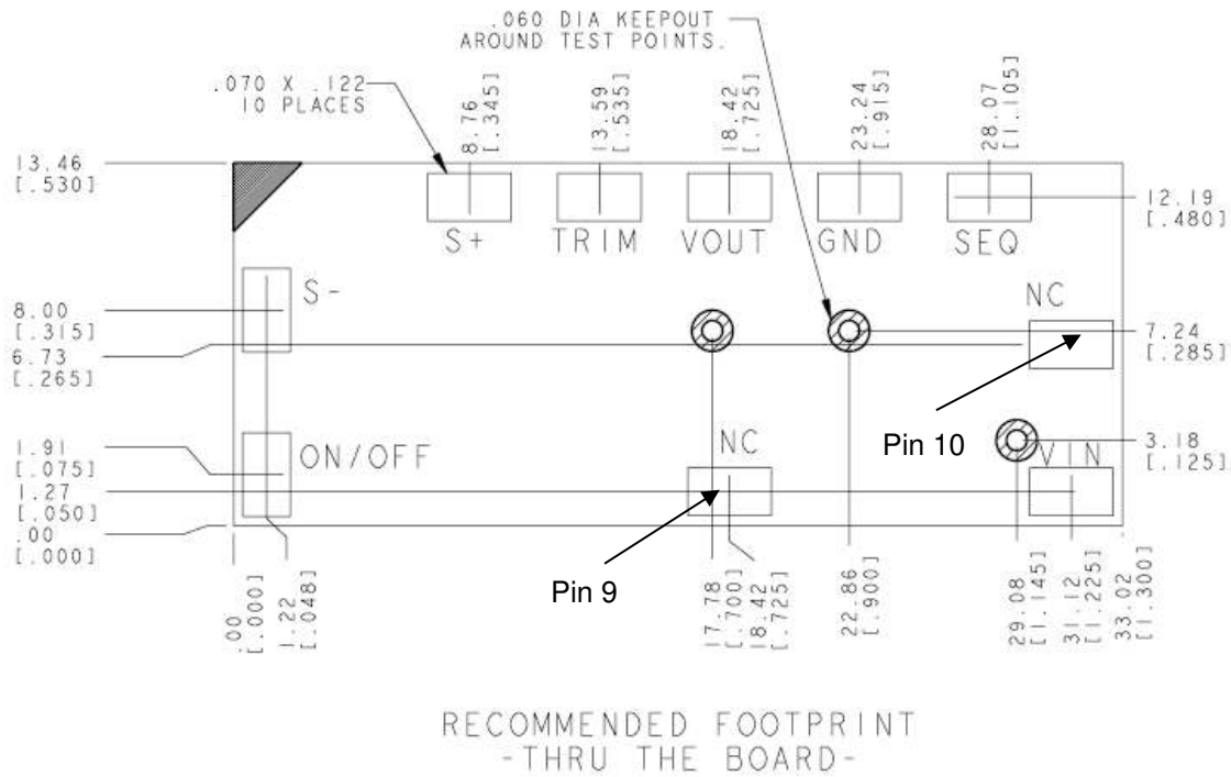
Figure 49. Recommended pad layout
