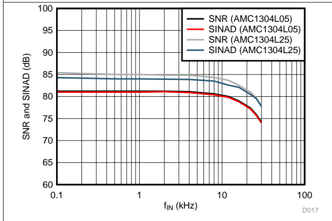
Figure 19. Signal-to-Noise Ratio and Signal-to-Noise + Distortion vs Input Signal Frequency
