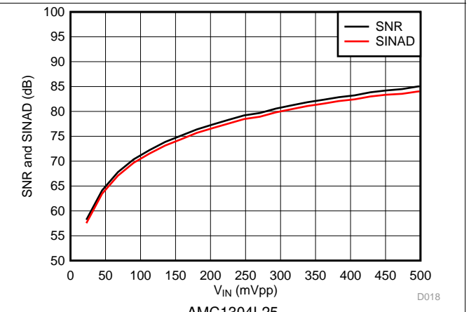
Figure 20. SNR and SINAD vs Input Signal Amplitude
