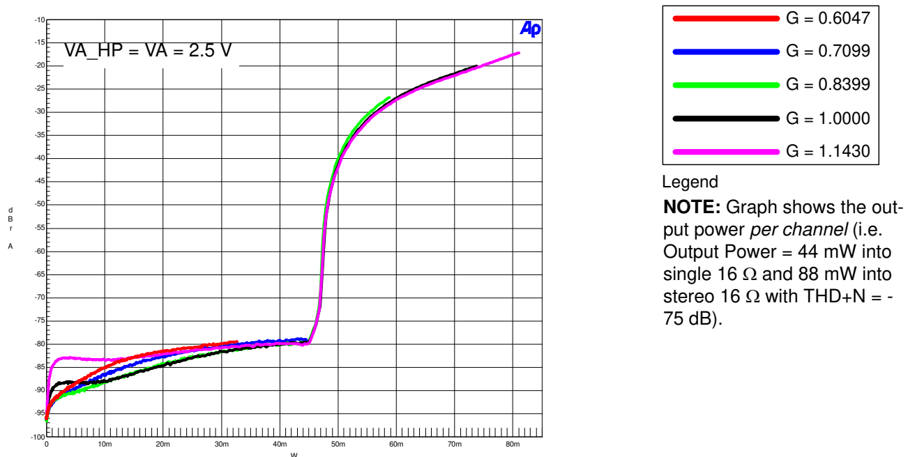
Figure 22. THD+N vs. Output Power per Channel at 2.5 V (16 \Omega load)
