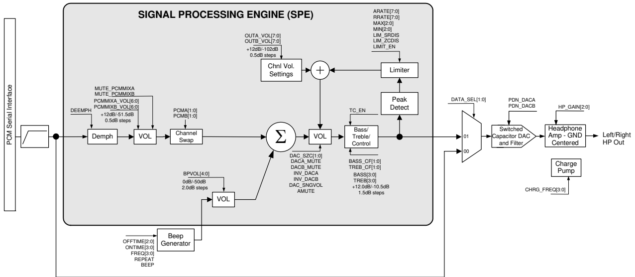
Figure 8. Output Architecture
