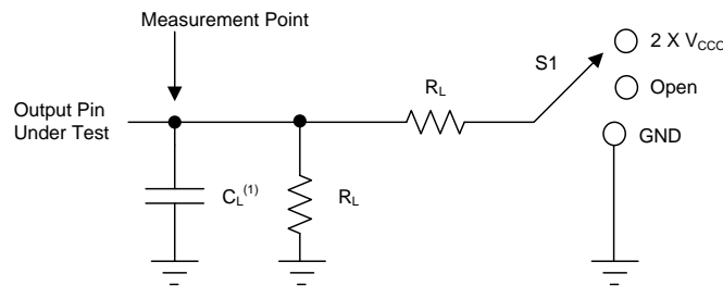
Figure 1. Load Circuit
