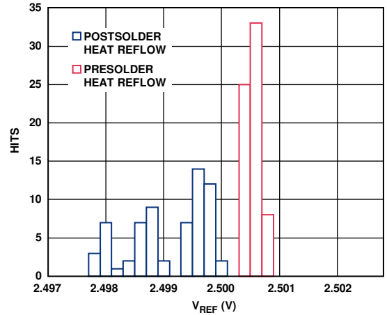
Figure 63. Solder Heat Reflow Reference Voltage Shift
