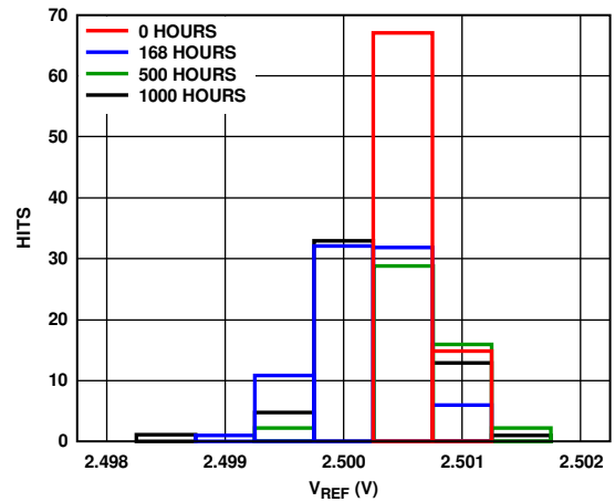
Figure 64. Reference Drift Through to 1000 Hours
