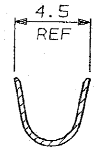
SECTION Y-Y
