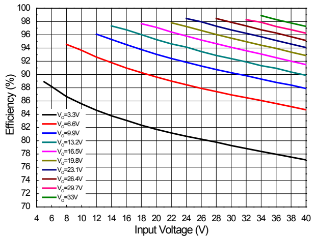
Efficiency vs. Input Voltage ( R_{SET} = 0.15\Omega , L = 47\mu\text{H} )
