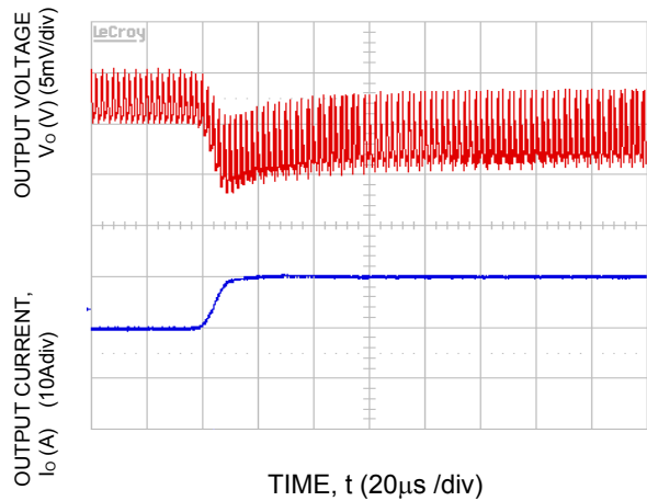
Fig-48. Transient Response to Dynamic Load Change from 50% to 100% at 12Vin, Cout= 1x47uF+11x330uF, CTune=47nF, RTune=178ohms
