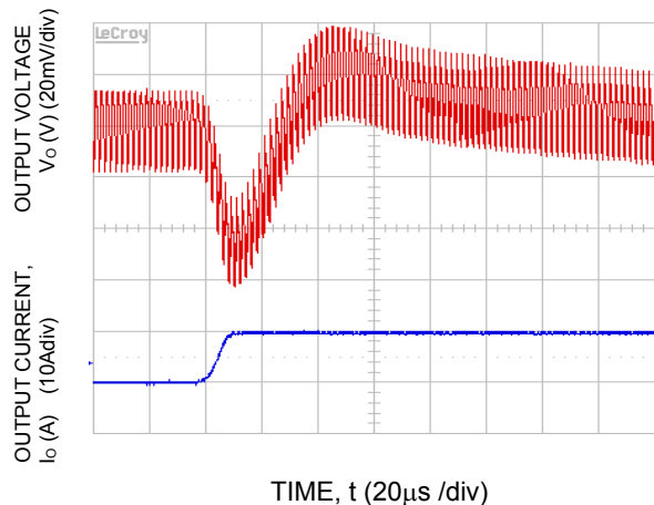
Fig-30. Transient Response to Dynamic Load Change from 50% to 100% at 12Vin, Cout= 2x47uF+2x330uF, CTune=3300pF & RTune=220ohms
