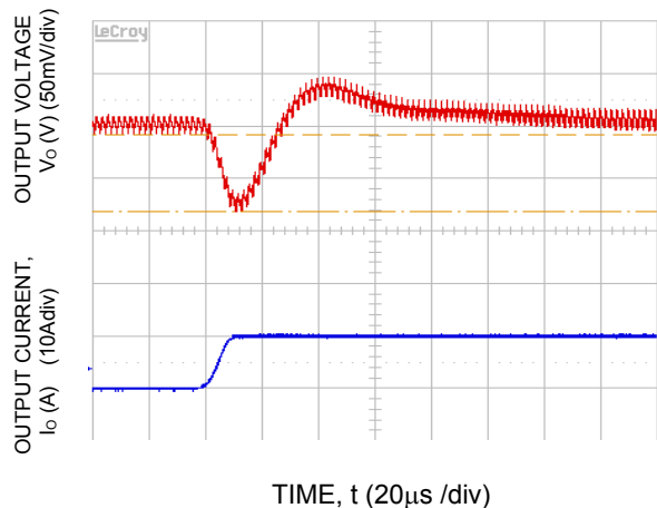
Fig-24. Transient Response to Dynamic Load Change from 50% to 100% at 12Vin, Cout= 5x47uF+1x330uF, CTune=2200pF & RTune=220ohms
