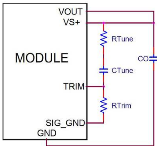
Fig-11: Circuit diagram showing connection of R_{TUNE} and C_{TUNE} to tune the control loop of the module.
