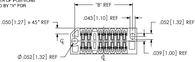
FIG 1 (MECF-08-01-XX-DV-XX SHOWN)
