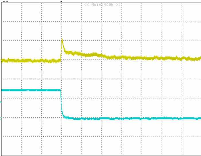
Figure 23: Typical transient response to step load change at 2.5A/\mu S from 50% to 0% of I_o , max at 5Vin, 1.8Vout (200uS/div) ( C_{out} = 47\mu F ceramic).top trace:Vout,0.1V/div;bottom trace:Iout:2A/div.
