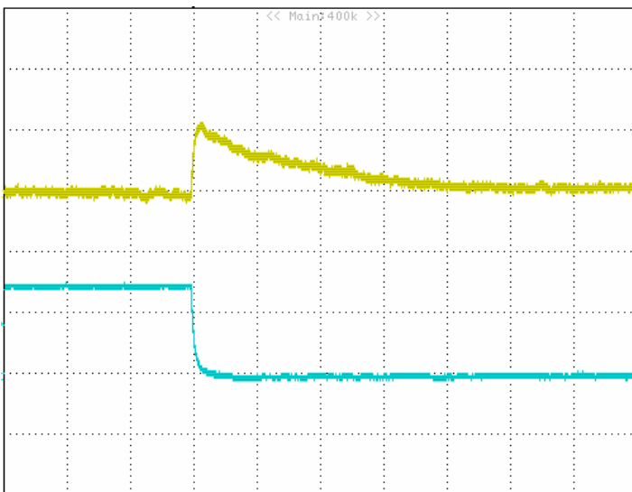
Figure 25: Typical transient response to step load change at 2.5A/\mu S from 50% to 0% of I_o , max at 5Vin, 3.3Vout (200uS/div) ( C_{out} = 47\mu F ceramic).top trace:Vout,0.1V/div;bottom trace:Iout:2A/div.
