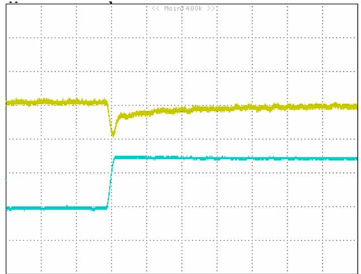
Figure 24: Typical transient response to step load change at 2.5A/\mu S from 0% to 50% of I_o , max at 5Vin, 1.8Vout (200uS/div) ( C_{out} = 47\mu F ceramic).top trace:Vout,0.1V/div;bottom trace:Iout:2A/div.
