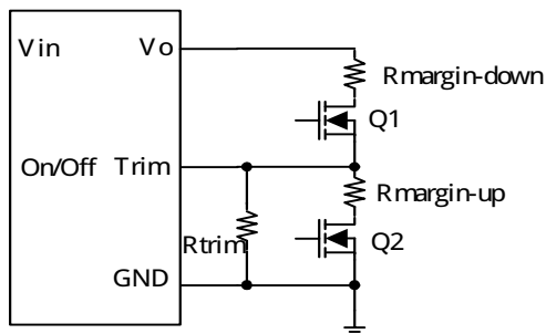
Figure 37: Circuit configuration for output voltage margining
