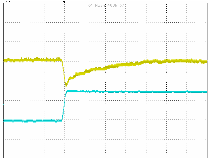
Figure 26: Typical transient response to step load change at 2.5A/\mu S from 0% to 50% of I_o , max at 5Vin, 3.3Vout (200uS/div) ( C_{out} = 47\mu F ceramic).top trace:Vout,0.1V/div;bottom trace:Iout:2A/div.
