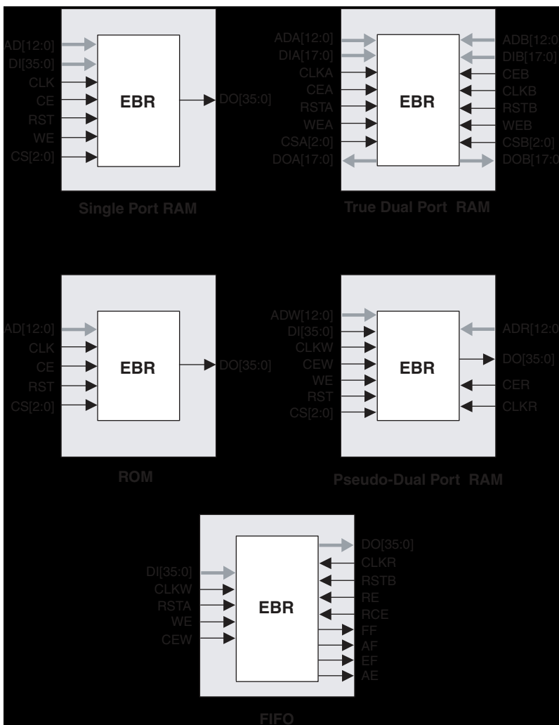
Figure 2-12. sysMEM Memory Primitives
