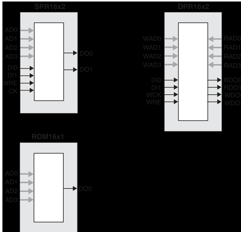
Figure 2-6. Distributed Memory Primitives
