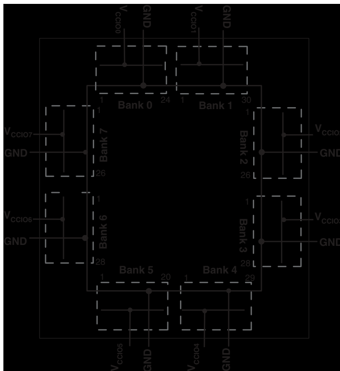
Figure 2-19. LA-MachXO1200 Banks
