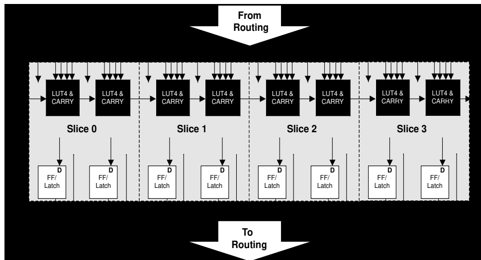
Figure 2-4. PFU Diagram
