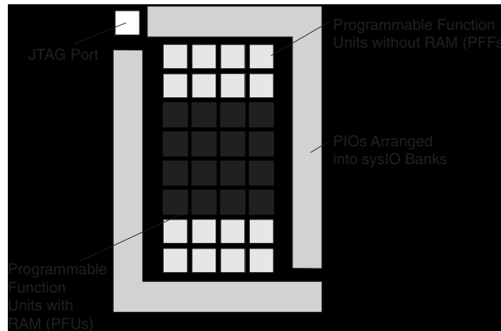
Figure 2-3. Top View of the LA-MachXO256 Device
