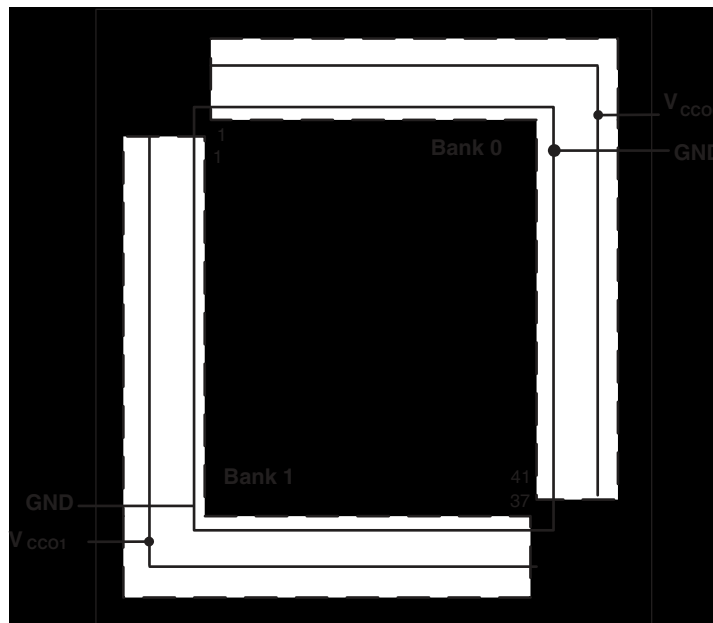
Figure 2-21. LA-MachXO256 Banks
