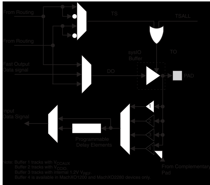
Figure 2-17. LA-MachXO PIO Block Diagram
