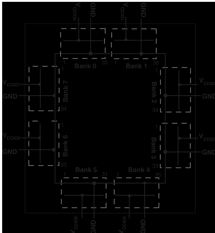
Figure 2-19. LA-MachXO1200 Banks
