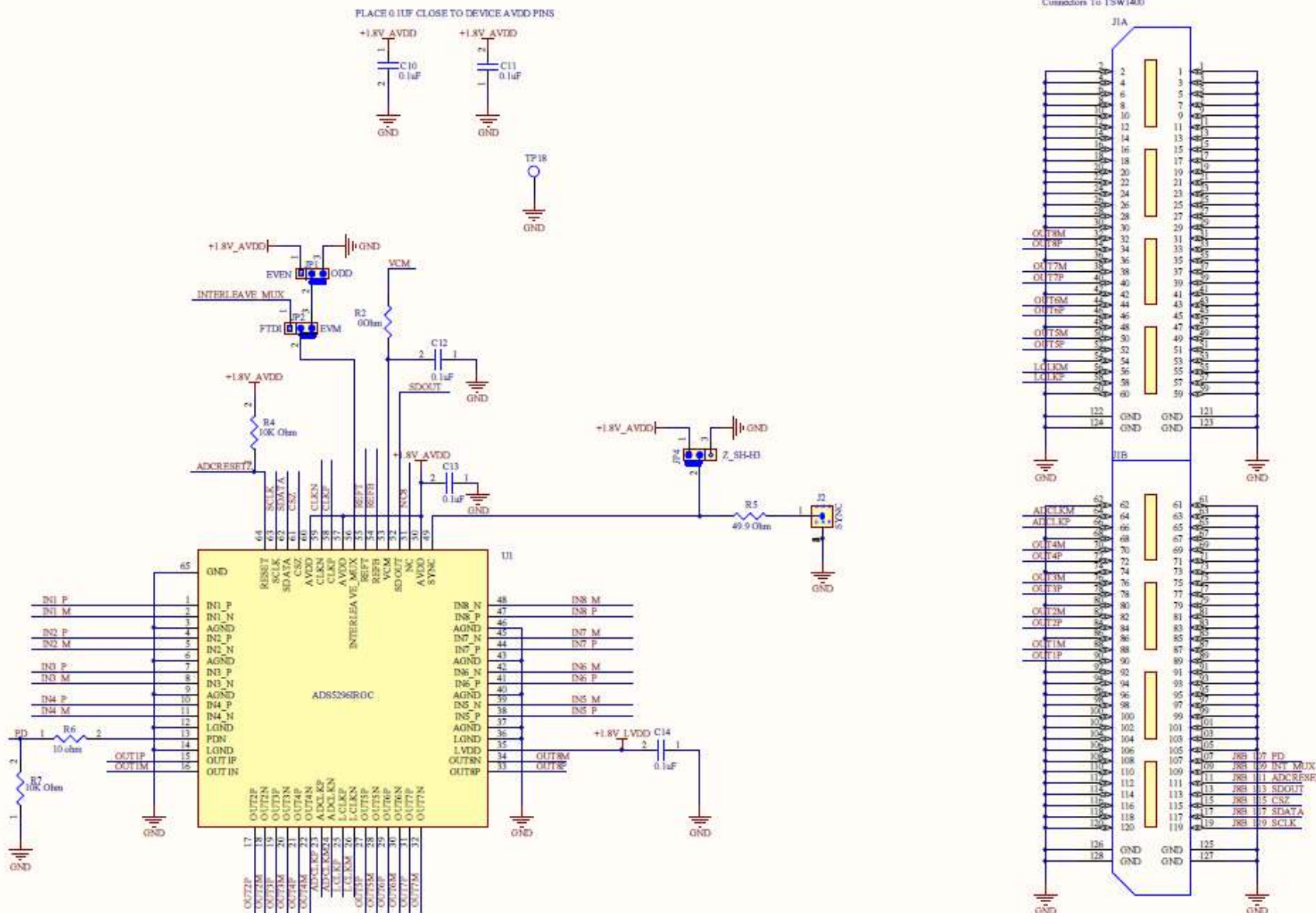
Figure 64. PGA5807 Schematic, (Sh. 2 of 16), ADS5296 Device
