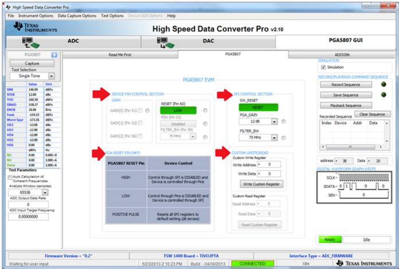
Figure 56. PGA5807 tab
