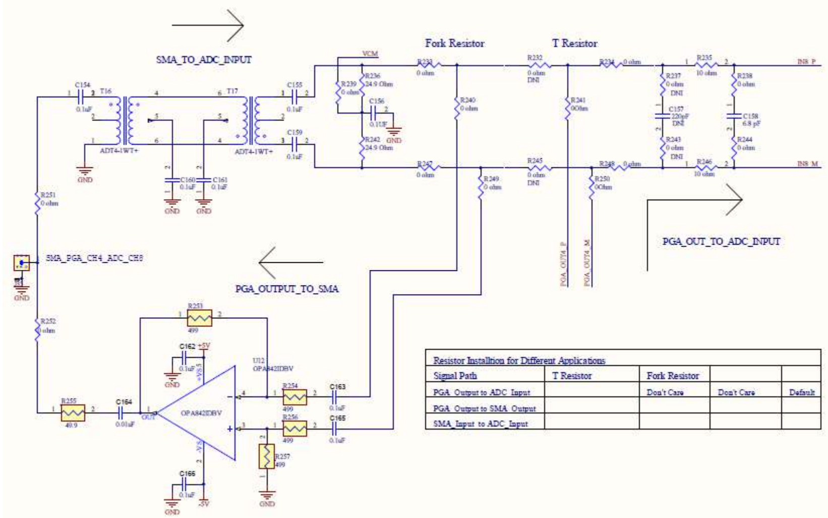
Figure 71. PGA5807 Schematic, (Sh. 9 of 16), PGA_CH4, ADC_CH8
