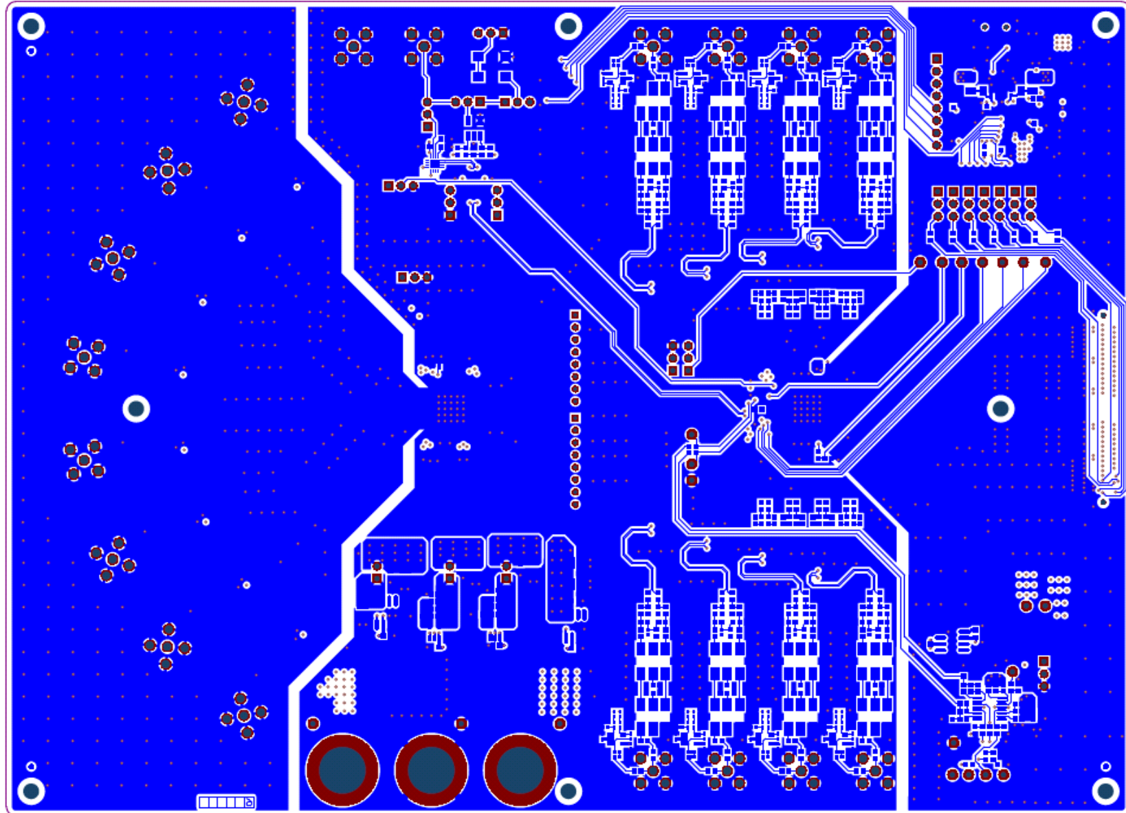
Figure 86. PGA5807 EVM Bottom Side
