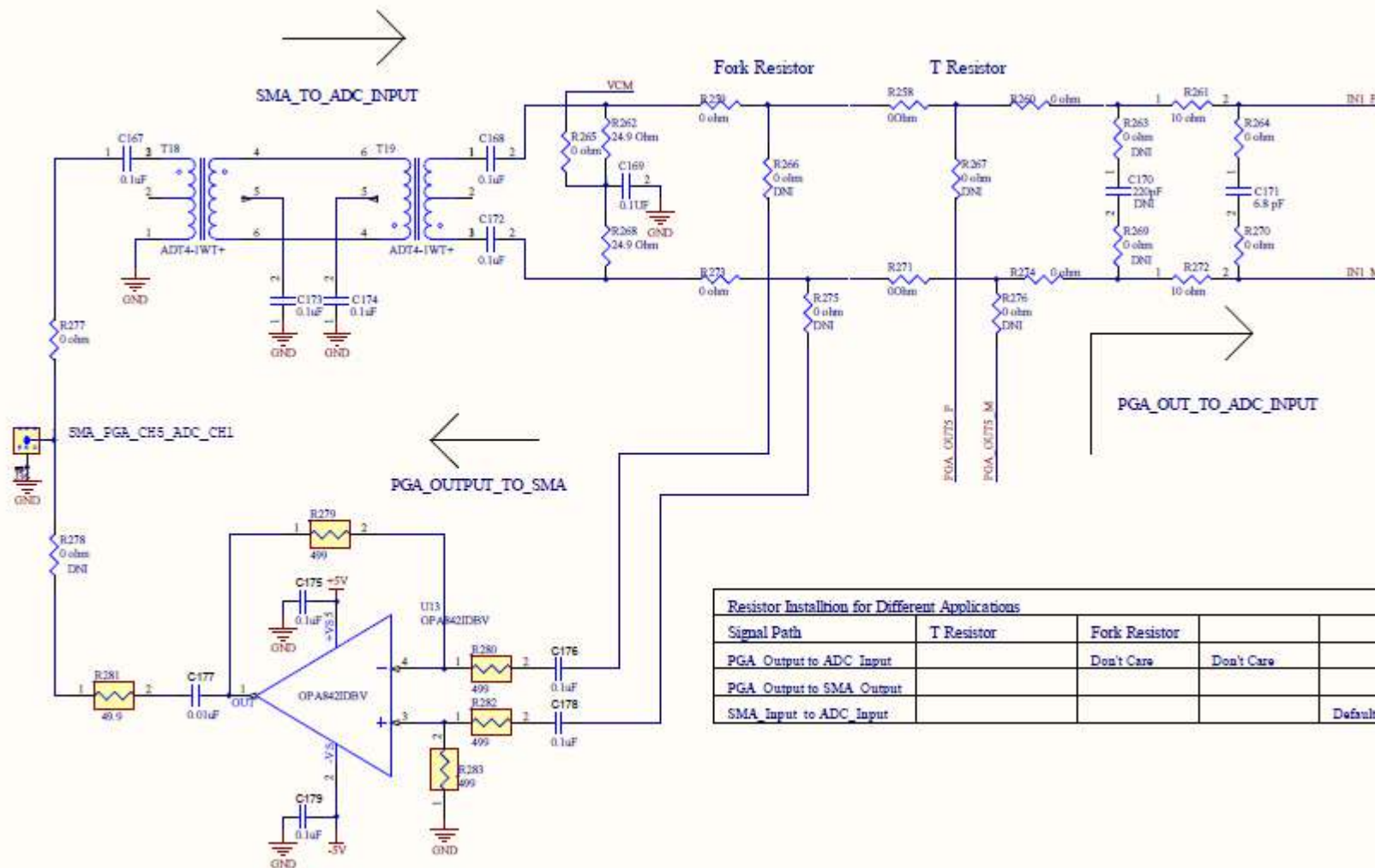
Figure 72. PGA5807 Schematic, (Sh. 10 of 16), PGA_CH5, ADC_CH1
