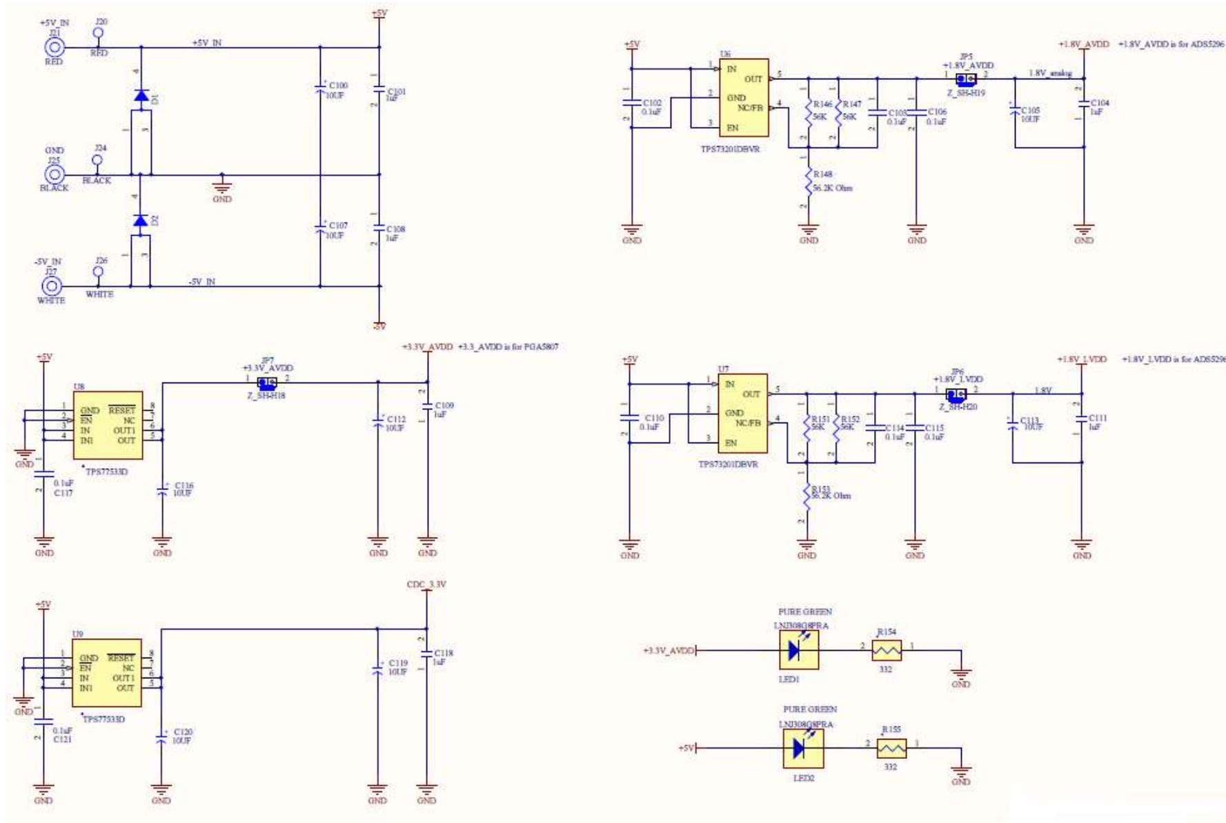
Figure 78. PGA5807 Schematic, (Sh. 16 of 16), Power Supply
