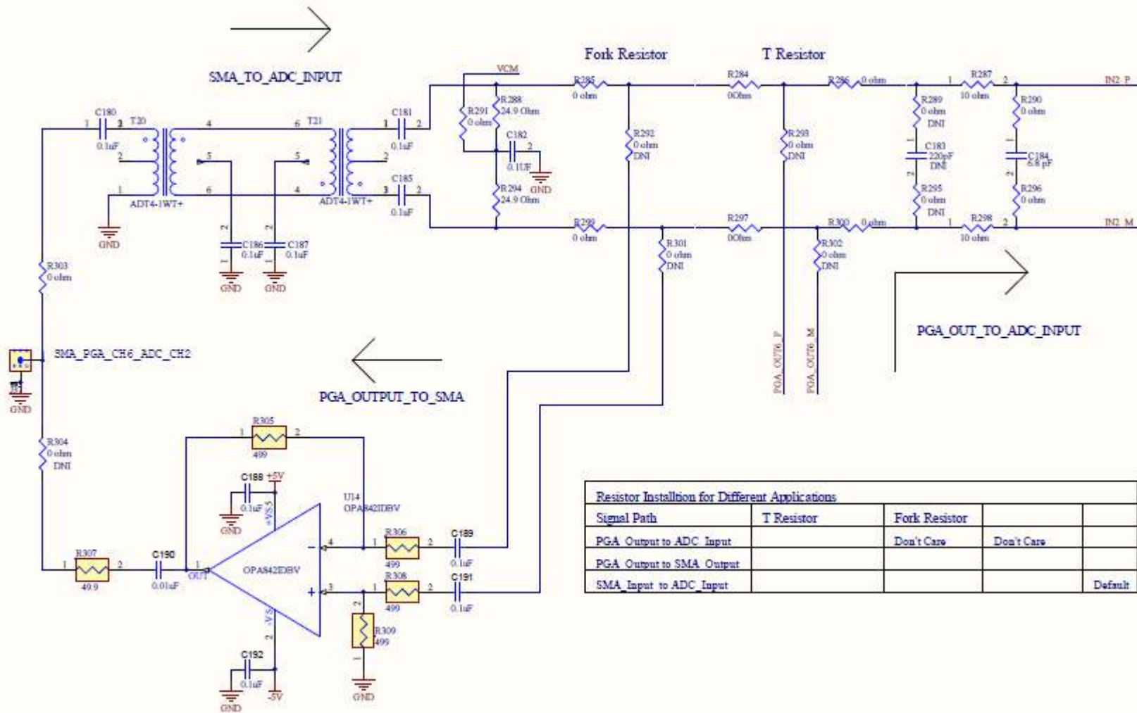
Figure 73. PGA5807 Schematic, (Sh. 11 of 16), PGA_CH6, ADC_CH2
