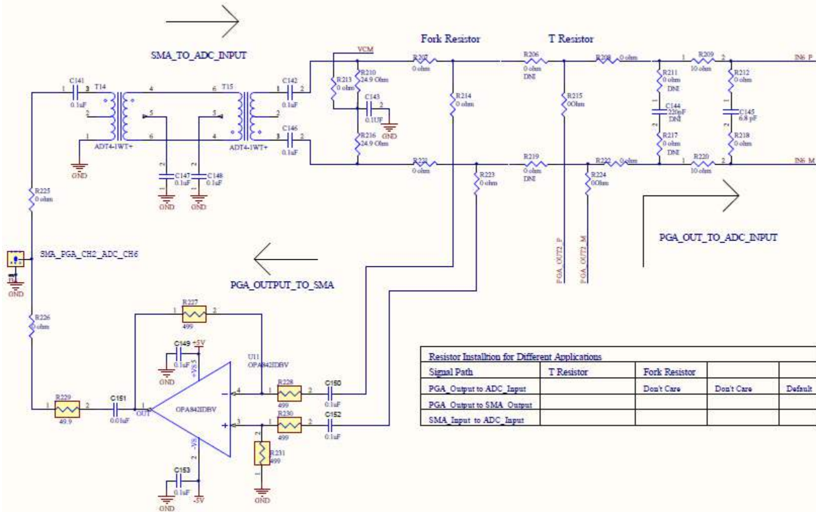
Figure 69. PGA5807 Schematic, (Sh. 7 of 16), PGA_CH2, ADC_CH6
