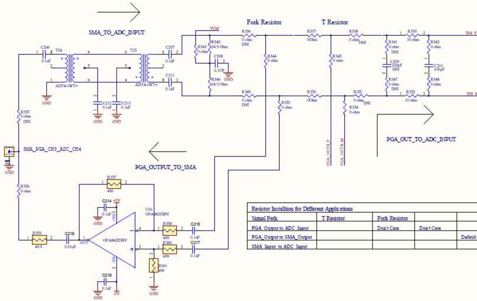
Figure 75. PGA5807 Schematic, (Sh. 13 of 16), PGA_CH8, ADC_CH4
