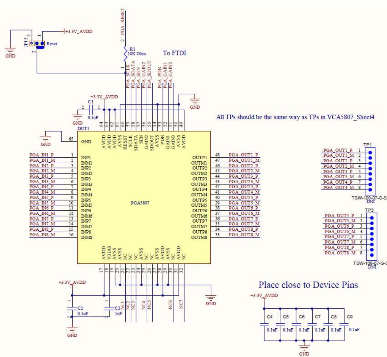
Figure 63. PGA5807 Schematic, (Sh. 1 of 16), PGA5807 Device
