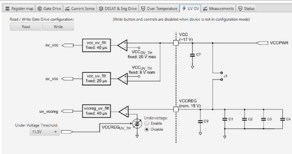
Figure 29. Undervoltage and overvoltage tab
