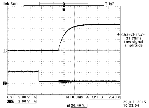
Figure 21. Vin = 24 V, Full Load startup from Enable CH1 = Vout CH3 = Enable
