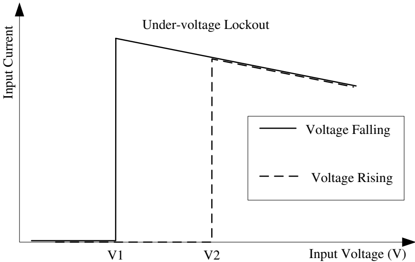
Figure 28. Input under-voltage lockout V_1 = 8\text{ V} V_2 = 10\text{ V}
