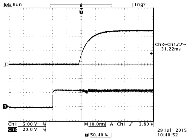
Figure 20. Vin = 24 V, Full Load startup from Vin CH1 = Vout CH3 = Vin
