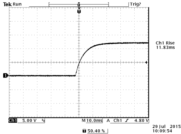
Figure 19. Rise time @ Vin = 24 V, Full Load
