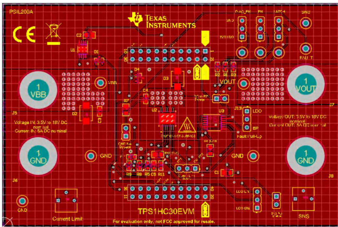
Figure 7-1. Top Layer
