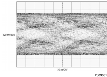
FIGURE 7. 6.25 Gb/s, PRBS-10 Input Signal to Equalizer after 30" of FR4
