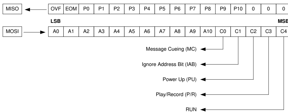
FIGURE 4: SPI PORT
