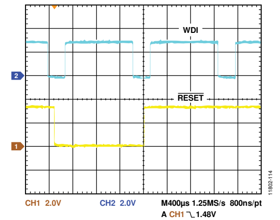
Figure 12. Fast Watchdog Timeout Period, Watchdog Timeout Option A
