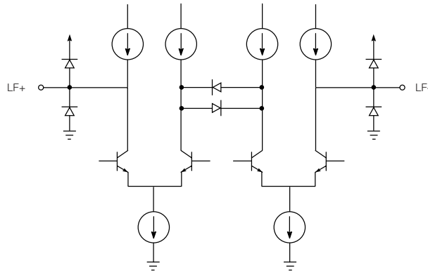
Figure 2-4: Loop Filter
