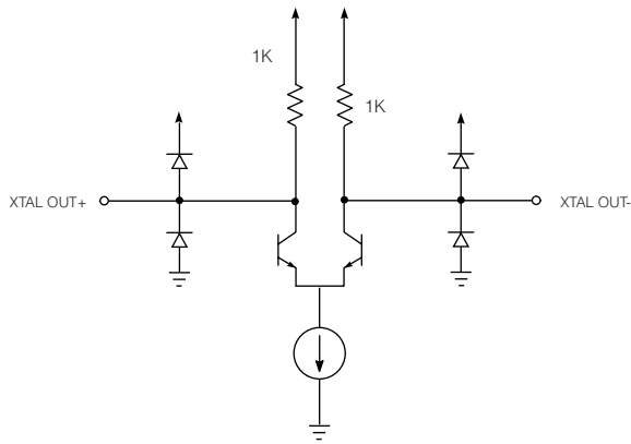
Figure 2-5: Crystal Output Buffer
