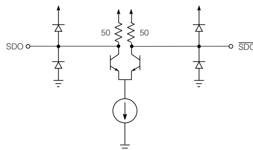
Figure 2-3: Serial Data Outputs
