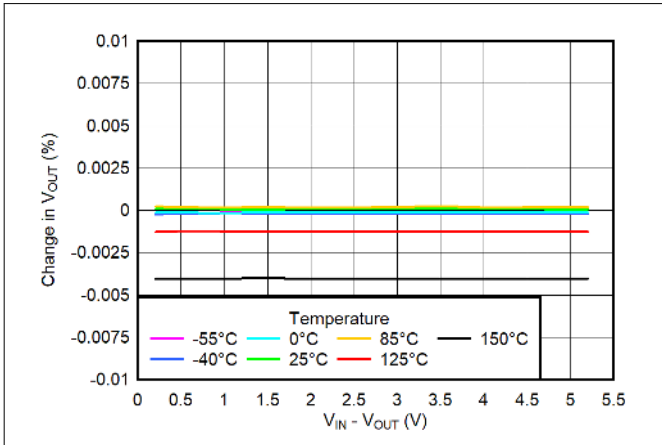
Figure 6-23. V IN Line Regulation
