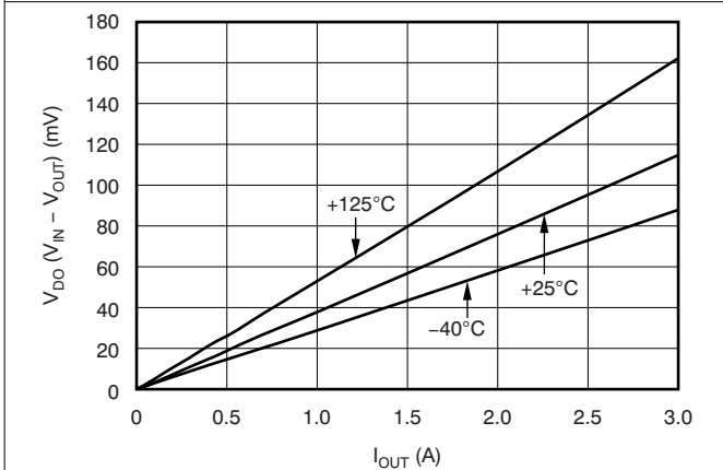
Figure 6-5. V_{IN} Dropout Voltage vs I_{OUT} and Temperature ( T_J )
