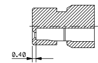
SECT J-J
