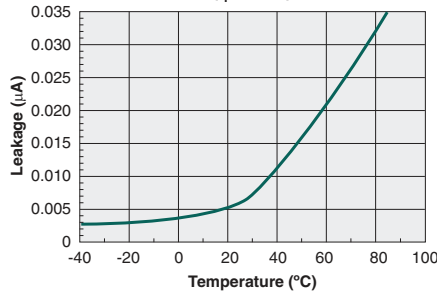
Form-B Typical Leakage vs. Temperature Measured across Pins 7&8 ( I_F=5mA )
