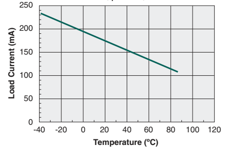
Form-B Maximum Load Current vs. Temperature ( I_F=0mA )
