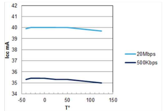
Figure 16. Driver I_{CC} vs temperature 60 \Omega load
