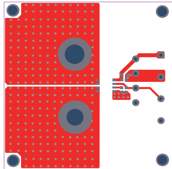
Figure 3: Top Layer
