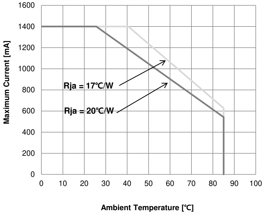
Fig 9. Maximum Forward Current vs. Ambient Temperature, T_{jmax} = 125^{\circ}C
