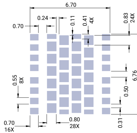
Recommended 6-V & 12-V Stencil Openings
