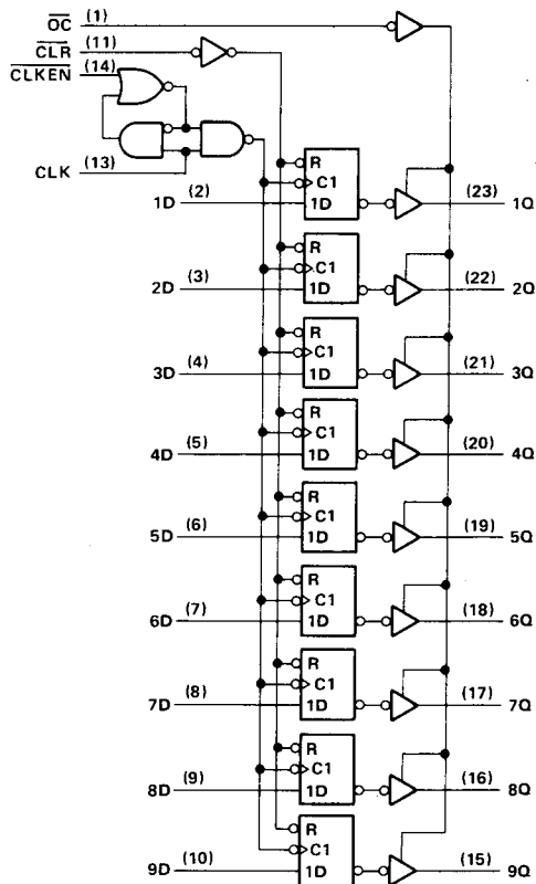
'ALS29823 logic diagram (positive logic)
