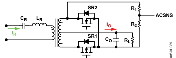
Figure 41. Resonant Synchronous Rectifier Control Circuit
