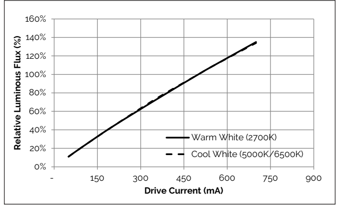
Figure 2: Relative Flux vs. Drive Current, T_c = 25^\circ\text{C}
