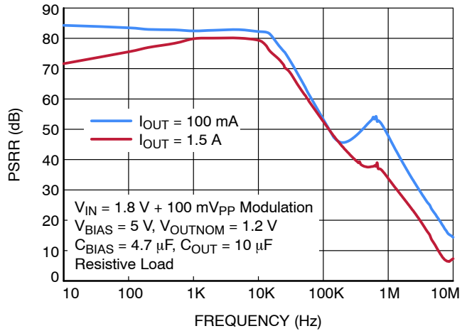
Figure 18. V_{IN} PSRR
