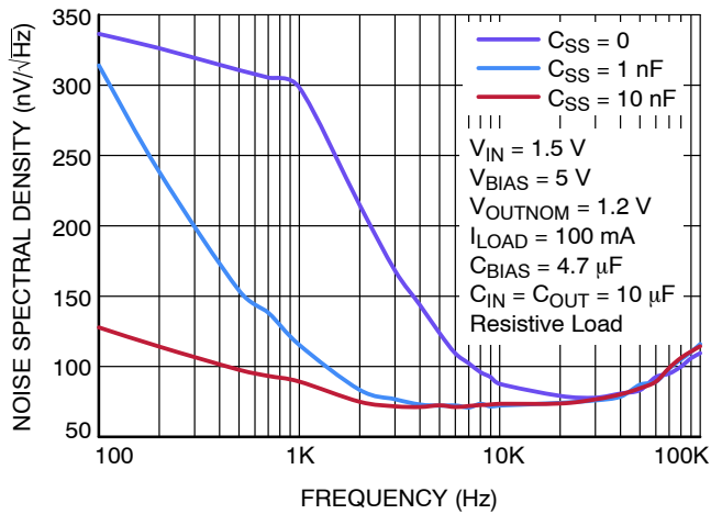
Figure 20. Noise Density vs. C_{SS}
