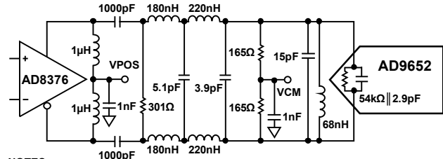
Figure 55. Differential Input Configuration Using the AD8376
