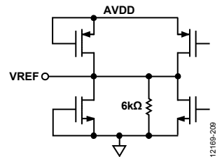
Figure 51. Equivalent VREF Circuit
