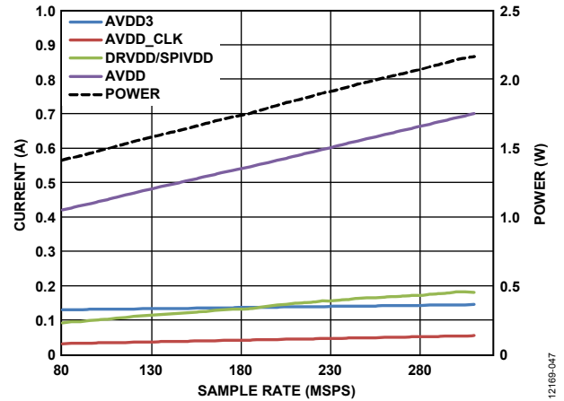
Figure 65. Power and Current vs. Sample Rate
