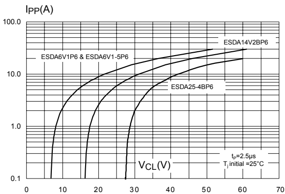
Figure 5. Clamping voltage versus peak pulse current ( T_j \text{ initial} = 25^\circ\text{C} , rectangular waveform, t_p = 2.5 \mu s )
