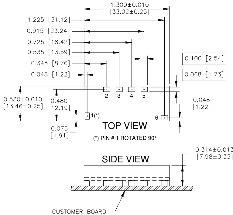
YNS05S Pinout (Surface Mount)
