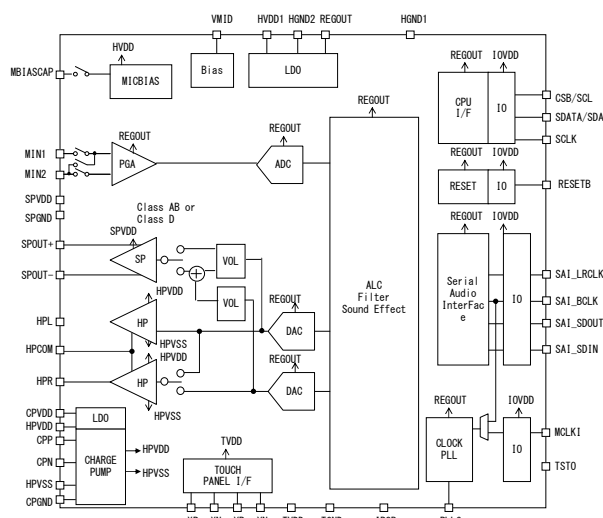
Figure 1. Block Diagram
