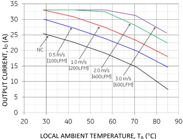
Figure 20. Output Current Derating for the Base plate QBDW033A0B-H at 48V in with Transverse airflow from Vin(-) to Vin(+)
