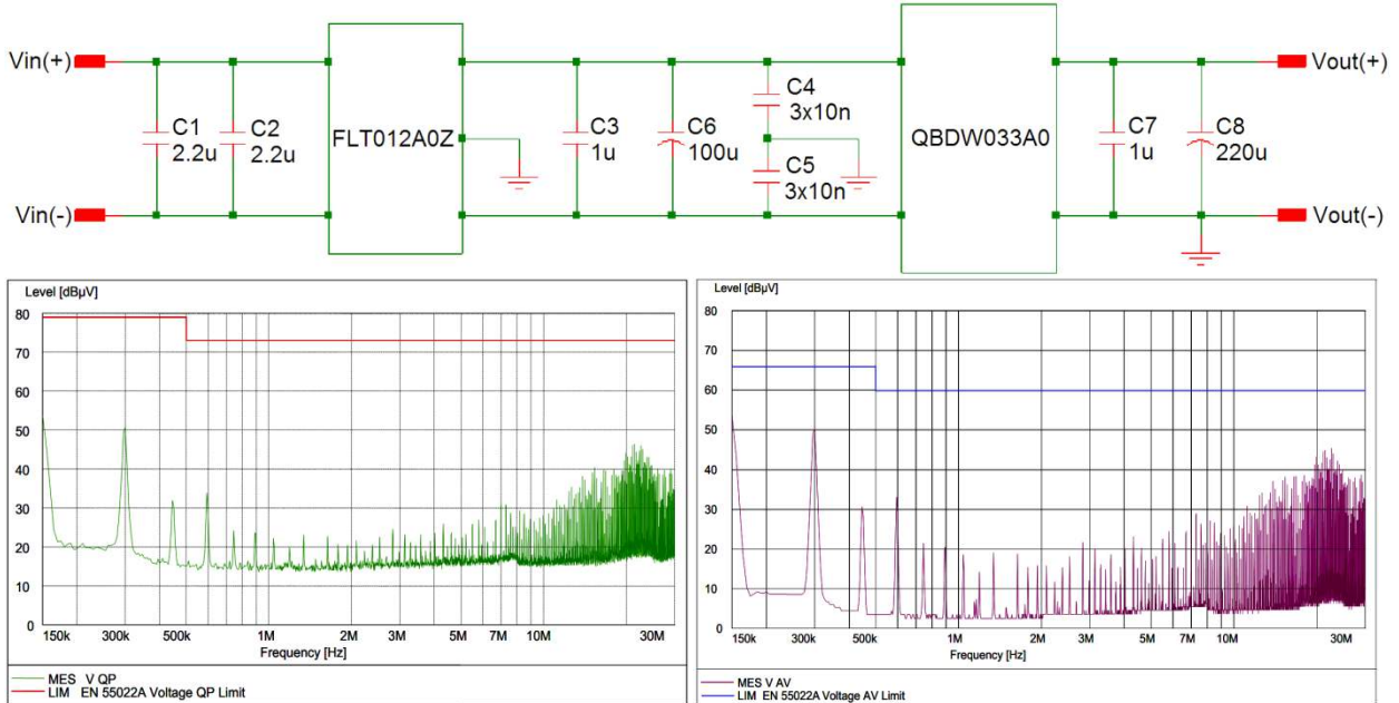
Figure 25. EMC Consideration
