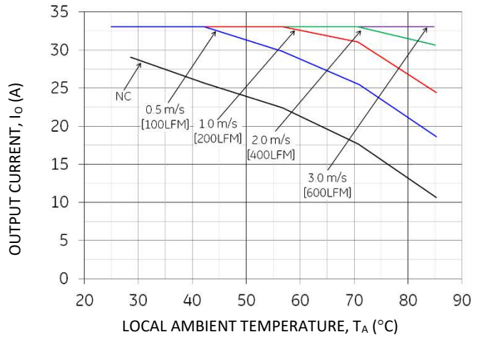
Figure 22. Output Current Derating for the Base plate QBDW033A0B-H at 48V in with 0.5 inch heatsink and Transverse airflow from Vin(-) to Vin(+)
