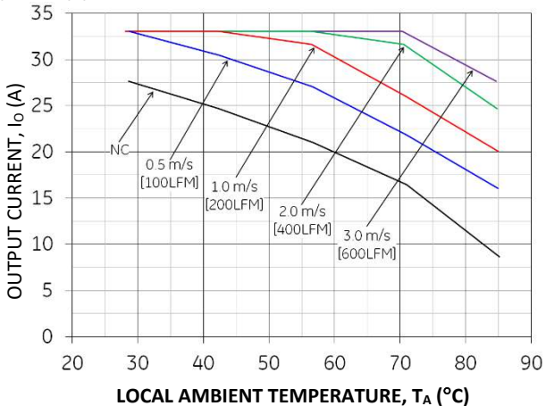
Figure 21. Output Current Derating for the Base plate QBDW033A0B-H at 48V in with 0.25 inch heatsink and Transverse airflow from Vin(-) to Vin(+)
