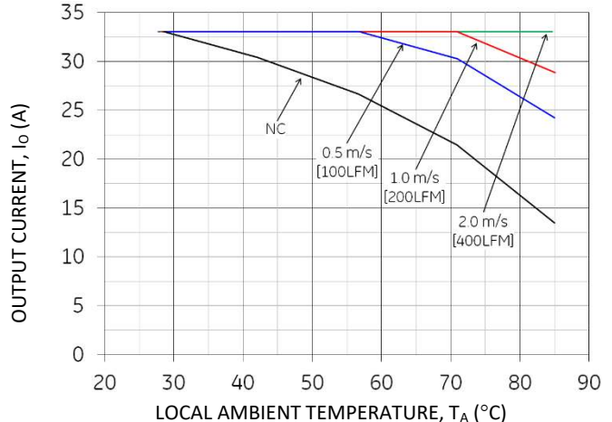
Figure 23. Output Current Derating for the Base plate QBDW033A0B-H at 48V in with 1.0 inch heatsink and Transverse airflow from Vin(-) to Vin(+)
