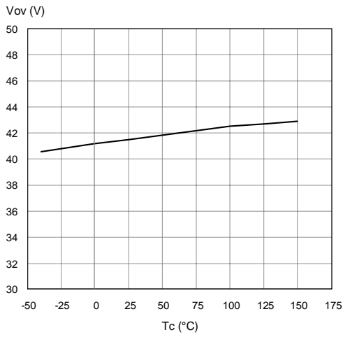
Figure 16. Overvoltage Shutdown
