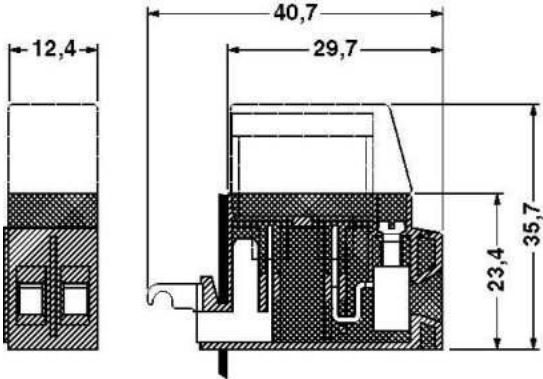
Dimensioned drawing
