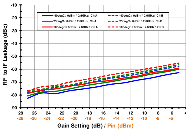
RF to IF Leakage [v Temp]
