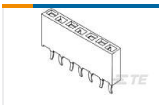
TE Part #215300-3 3P HV100 REC CON. TE, 8.5MM,TIN
