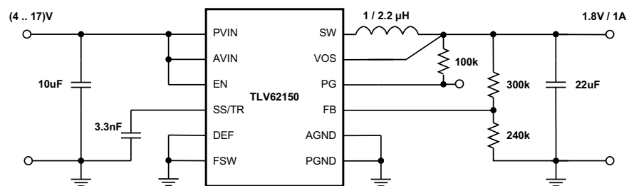
Figure 42. 1.8-V/1-A Power Supply
