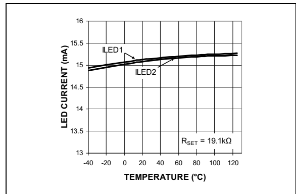
FIGURE 2-6: LED Current vs. Temperature.
