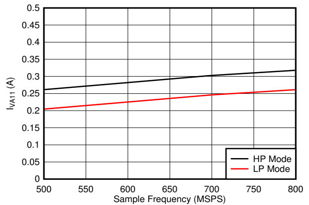
Independent of JMODE Figure 7-96. Single Channel, I_{VA11} vs F_S
