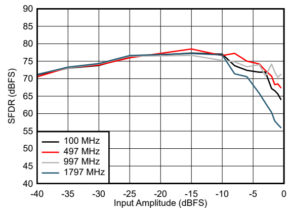
Figure 7-30. SFDR vs Input Amplitude Low Power Mode
