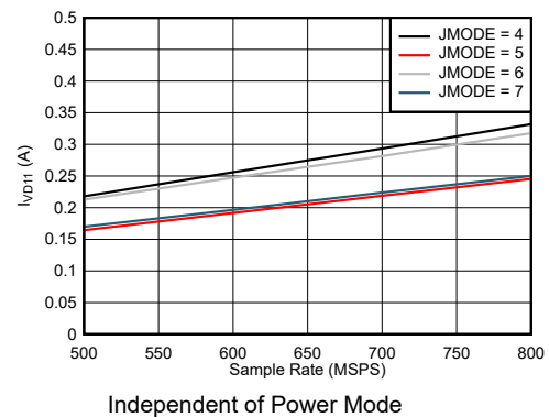
Figure 7-78. Quad Channel, I_{VD11} vs F_S for JMODES 4 - 7
