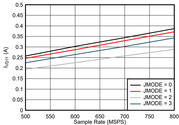
Independent of Power Mode Figure 7-77. Quad Channel, I_{VD11} vs F_S for JMODES 0 - 3
