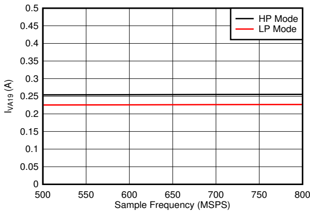
Independent of JMODE Figure 7-95. Single Channel, I_{VA19} vs F_S
