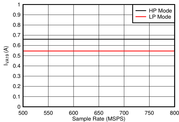
Independent of JMODE Figure 7-75. Quad Channel, I_{VA19} vs F_S
