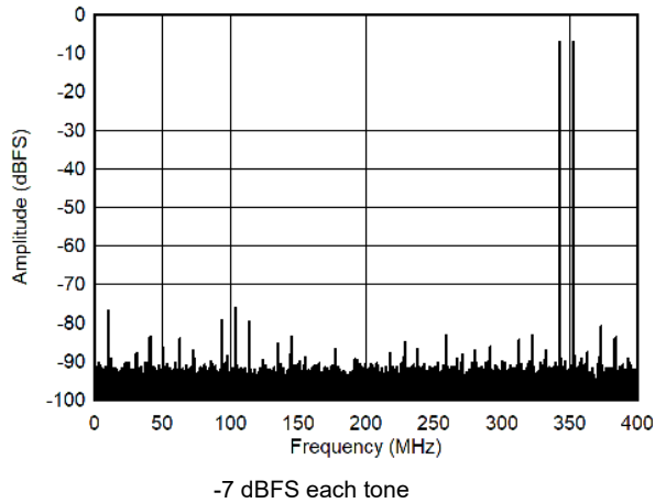
Figure 7-51. Single Tone FFT at 348 MHz
