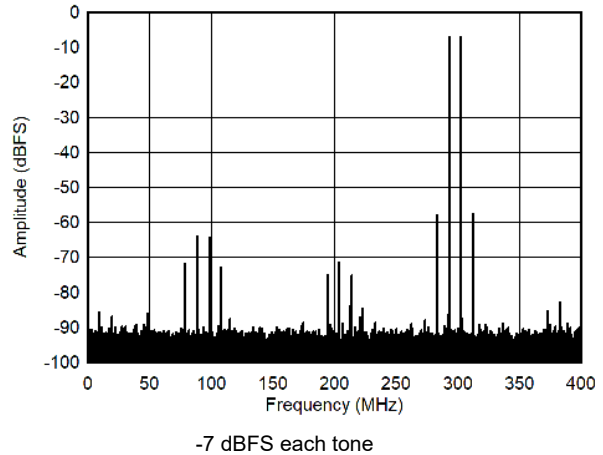
Figure 7-54. Single Tone FFT at 2698 MHz
