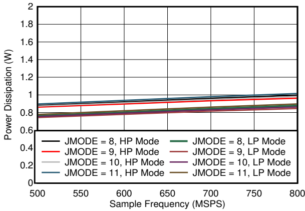
Figure 7-93. Single Channel, Power Dissipation vs F_S for JMODES 8 - 11
