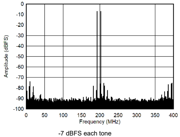
Figure 7-52. Single Tone FFT at 998 MHz
