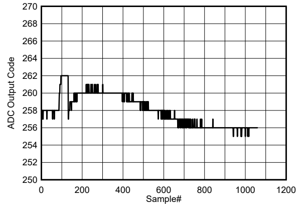
Figure 7-116. Background Core Transition (DC midscale input)
