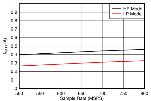
Independent of JMODE Figure 7-76. Quad Channel, I_{VA11} vs F_S
