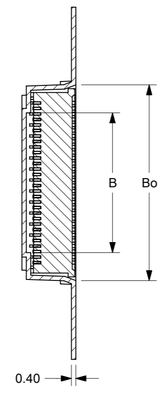
SECTION Y-Y
