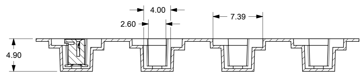
SECTION Z-Z
